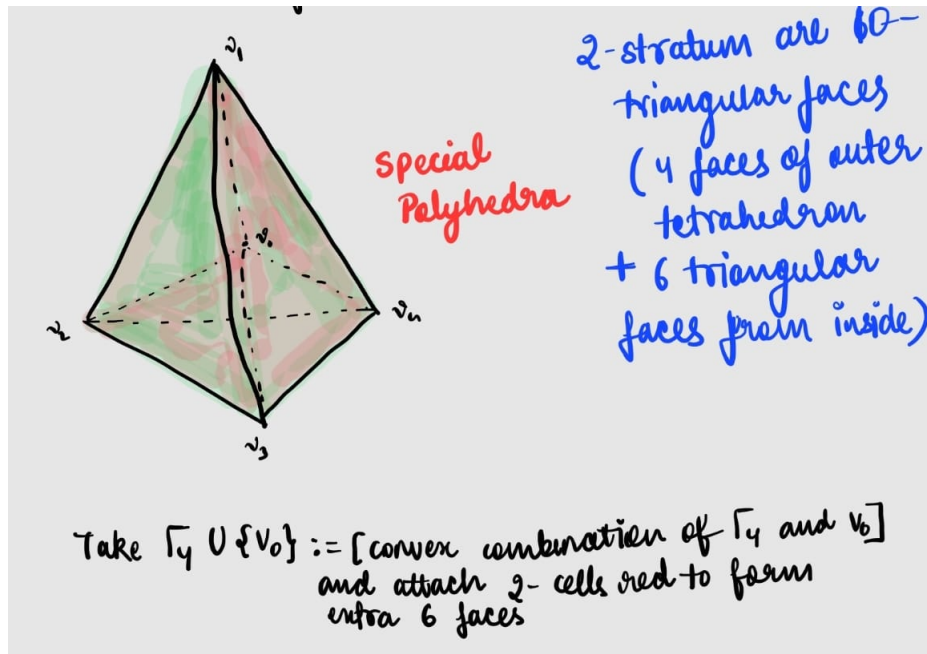
Figure 7: special polyhedron
